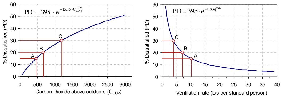
Figure7. Left: Carbon dioxide (CO 2 ) as indicator of human bio effluents [28,29]; Percentage of dissatisfied visitors as function of the CO 2 concentration above outdoor levels where sedentary occupants are the exclusive pollution sources. Right: Percentage of dissatisfied visitors as function of the ventilation rate per standard person (average sedentary office worker being thermally neutral, [29]). The pollution generated by such a standard person is called “olf”; the required minimum ventilation rate according to the three air quality categories A, B and C are 10 L/s.olf, 7 L/s.olf and 4L/s.olf, respectively.
